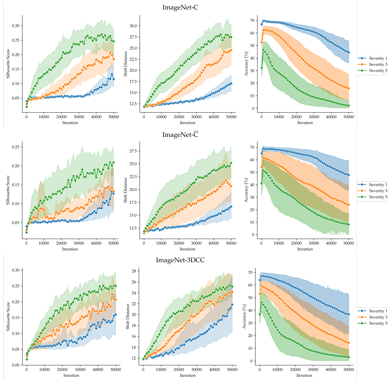
Figure 11. Changes in Silhouette scores, Shift distances, and Accuracies as Tent adapts to its inputs. We group together noises by severity level, and average the data for every iteration.
